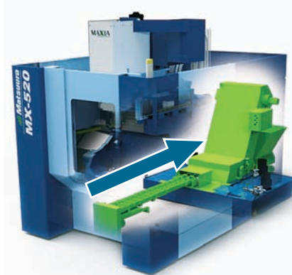
Spiral chip conveyor + Lift-up chip conveyor
