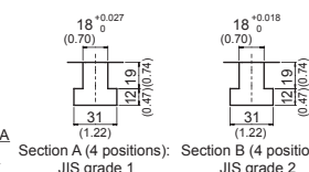
Centre hole details
