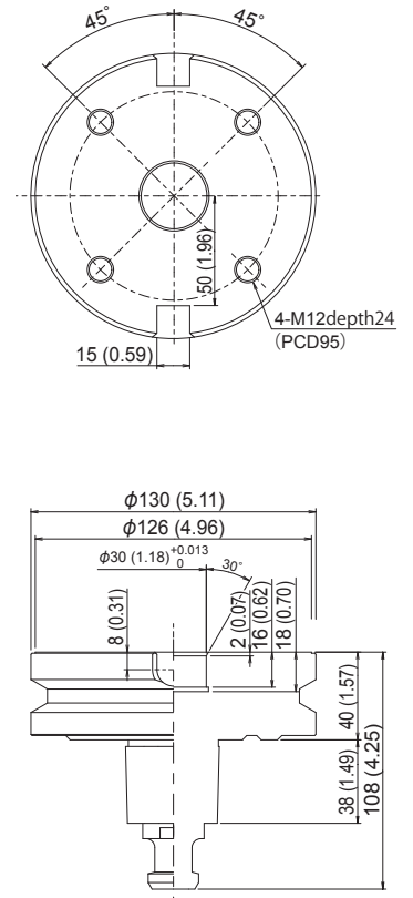
Pallet top view
