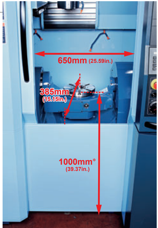
Minimal interference between the spindle head & table, offering excellent workpiece access to the cutting tool.
